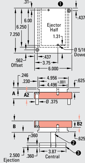
T-Style Solid or Laminated: 6.0 x 7.25
