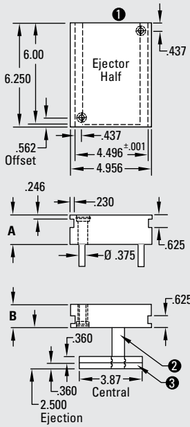
Standard Solid: 4.5 x 6.25
