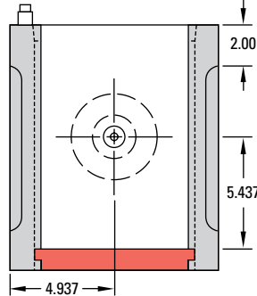
UF 321 Frame Lower – Side View
