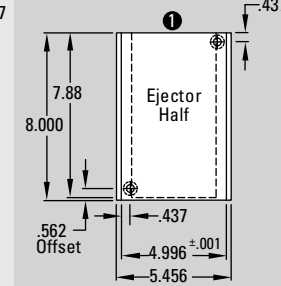
Standard Laminated: 5.0 x 8.0
