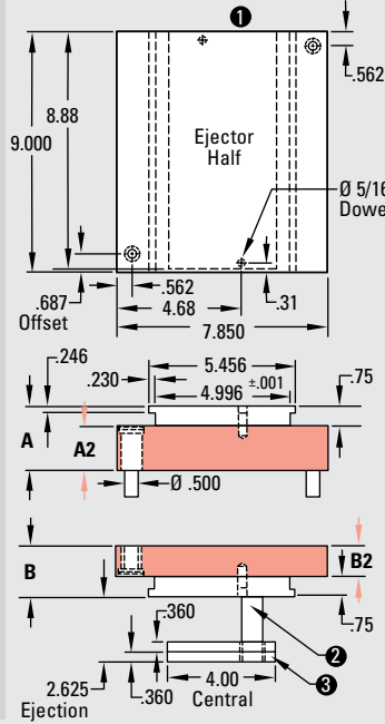
T-Style Solid or Laminated: 7.85 x 9.0
