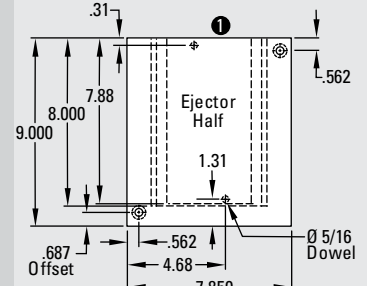
T-Style Solid or Laminated: 7.85 x 9.0
