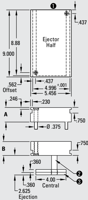
Standard Solid: 5.0 x 9.0
