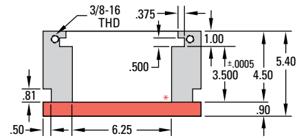
UF 321 Frame Lower – Side View
