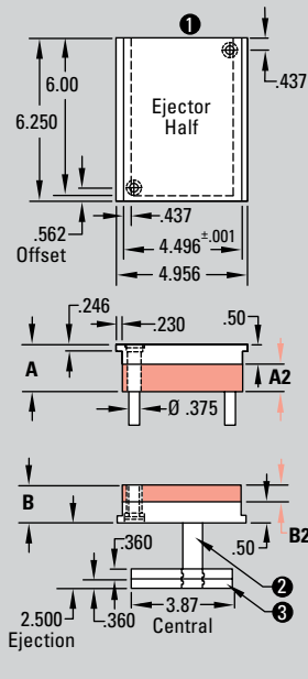
Standard Laminated: 4.5 x 6.25
