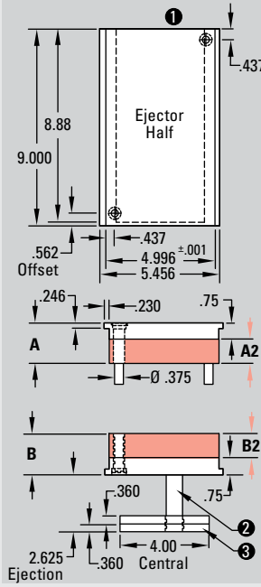
Standard Laminated: 5.0 x 9.0
