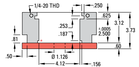
UF 321 Frame Lower – Side View
