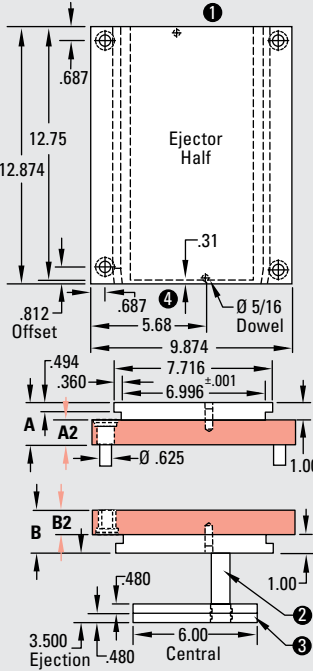
T-Style Laminated: 9.9 x 12.9
