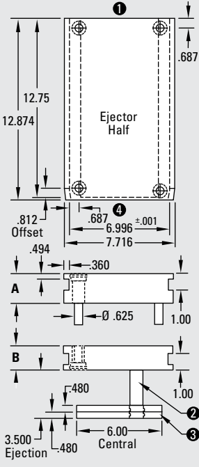
Standard Solid: 7.0 x 12.9
