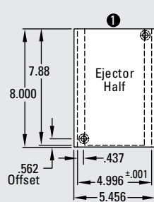
Standard Solid: 5.0 x 8.0
